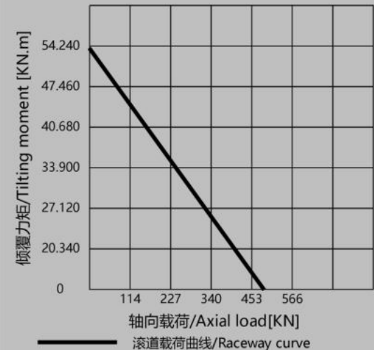
载荷曲线图/MOMENT LOAD CHART
