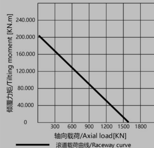
载荷曲线图/MOMENT LOAD CHART
